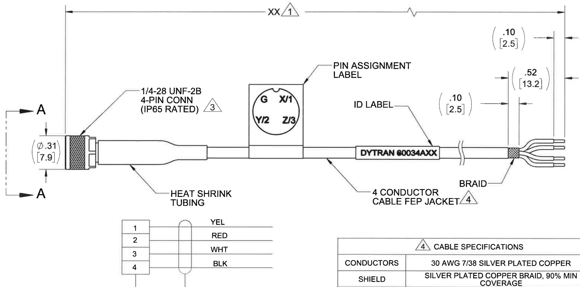
SCHEMATIC DIAGRAM
