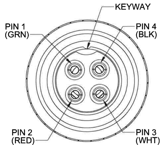
VIEW A-A SCALE 8 : 1
