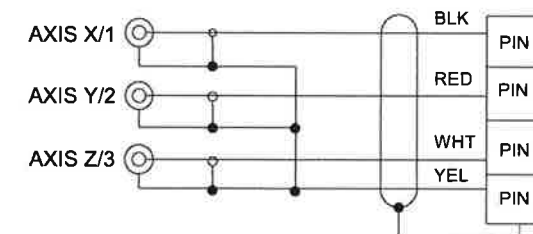
SCHEMATIC DIAGRAM
